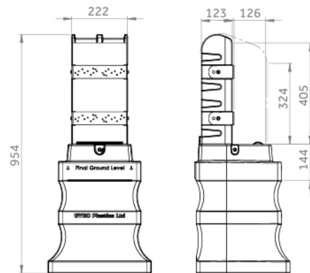
FUSE MOUNTING AREA MAXIMUM CAPACITY 12x FUSES
