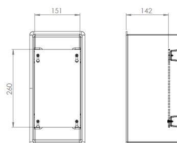
MOUNTING AREA DIMENSIONS
