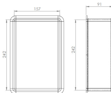
MOUNTING AREA DIMENSIONS
