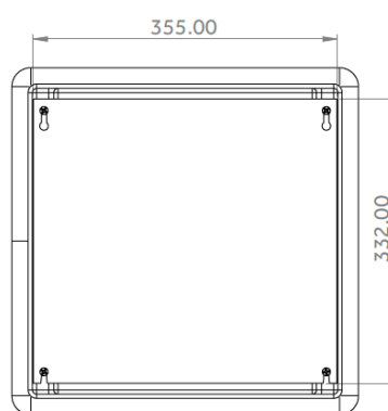
MOUNTING AREA DIMENSIONS
